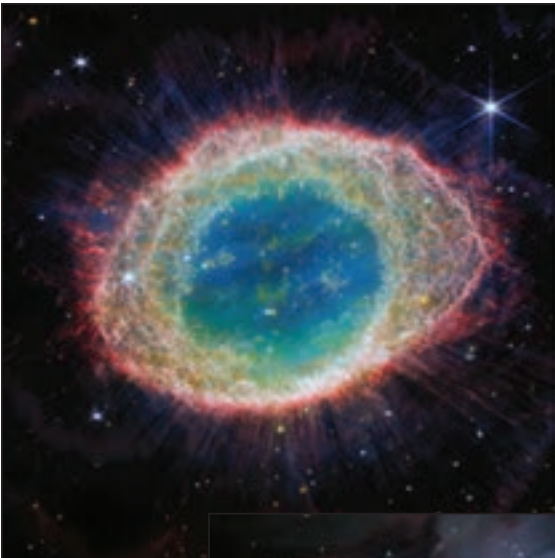
Look at the inner nebula These often take comparatively close-up views of the Ring Nebula. This is a smaller section of what was once a planetary nebula, a cloud of gas and dust that has been ejected from a star. The inner nebula is the core of the nebula, where the gas and dust are most concentrated. The outer nebula is the shell of the nebula, where the gas and dust are more spread out. The inner nebula is often a bright red or orange color, while the outer nebula is often a blue or white color. The inner nebula is often a ring shape, while the outer nebula is often a more diffuse, cloud-like shape.
