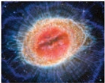
Look at the inner nebula These often take comparatively close-up views of the Ring Nebula. This is a smaller section of what was once a planetary nebula, a cloud of gas and dust that has been ejected from a star. The inner nebula is the core of the nebula, where the gas and dust are most concentrated. The outer nebula is the shell of the nebula, where the gas and dust are more spread out. The inner nebula is often a bright red or orange color, while the outer nebula is often a blue or white color. The inner nebula is often a ring shape, while the outer nebula is often a more diffuse, cloud-like shape.
